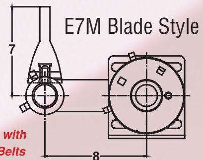
E12 Secondary Cleaner with E7M Blade
